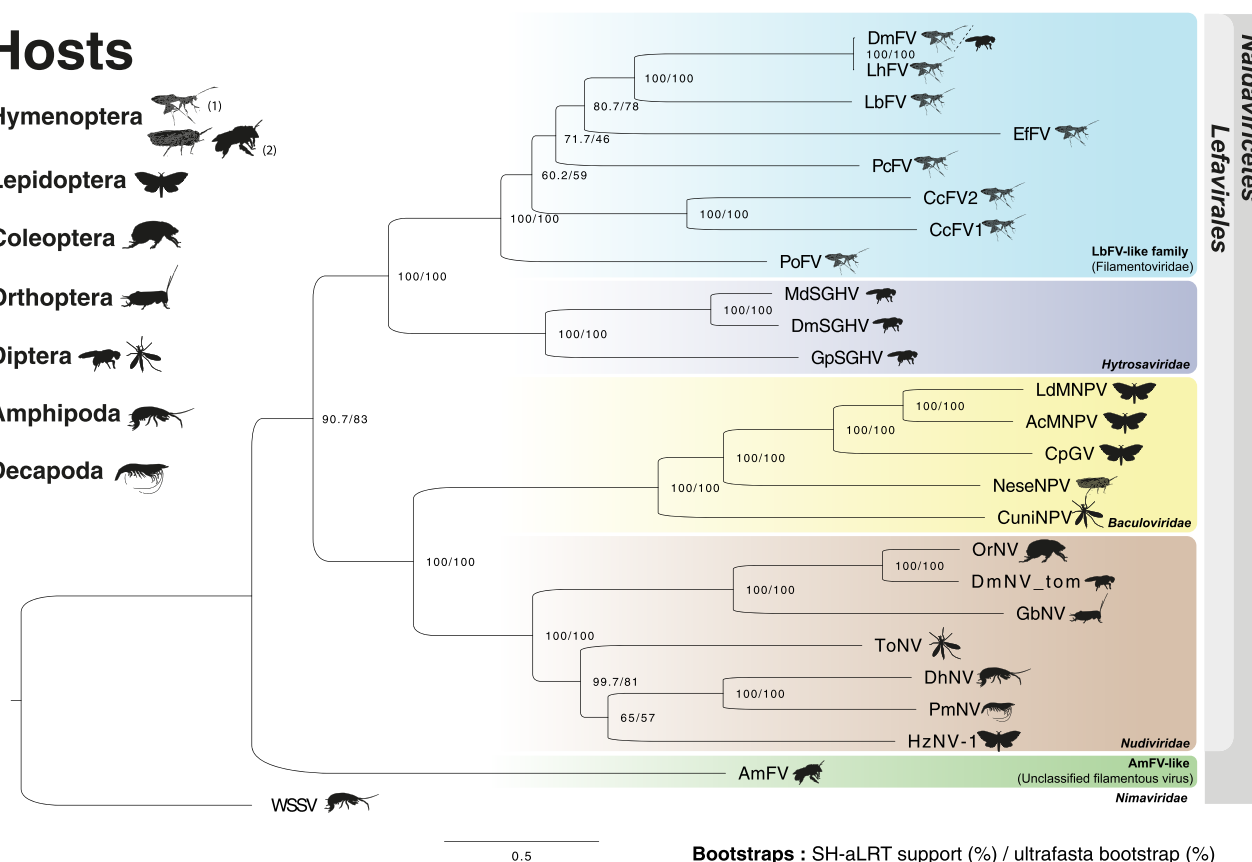
Figure 3. Phylogenetic tree of large dsDNA viruses from the Naldaviricetes class. Relationships were inferred using ML analysis in IQ-TREE v2 from twenty-five virus species with 17,114 sites with 16,650 distinct patterns at the amino-acid level. Bootstrap values are shown at each node (SH-aLRT support (%) / ultrafast bootstrap (%)). The scale bar indicates the average number of amino acid substitutions per site. Viral families are represented by the following colors: brown = Nudiviridae, yellow = Baculoviridae, purple = Hytrosaviridae, light blue = proposed Filamentoviridae and green = AmFV-like (Supplementary Tables S1 and S2). After each virus name a drawing represents the order of arthropod to which the infected host belongs. Hymenoptera have two lifestyle categories indicated: (1) endoparasitoids or (2) free-living species. DmFV and LhFV are likely the same virus infecting the Drosophila parasitoid L. heterotoma , although DmFV has been initially detected from a pool of wild-caught Drosophila (Section 2.5).
